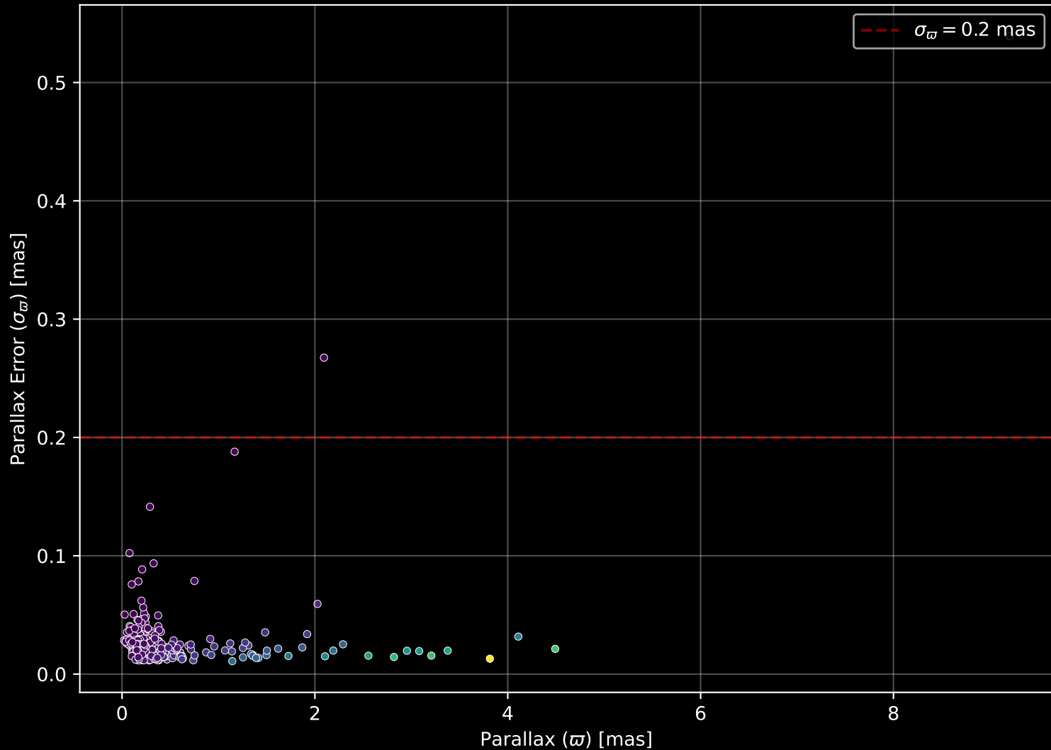
APOGEE DR17 Field: [140+06] Parallax Quality (n= 352)
