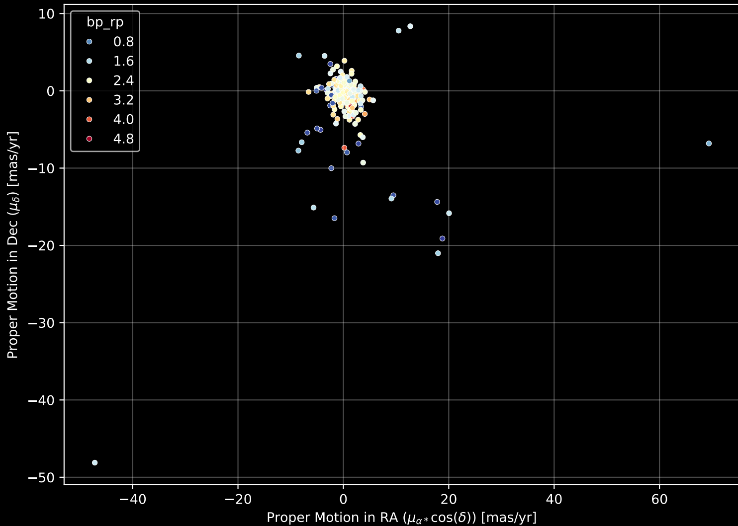
APOGEE DR17 Field: [140+06] Proper Motion Diagram (n= 352)
