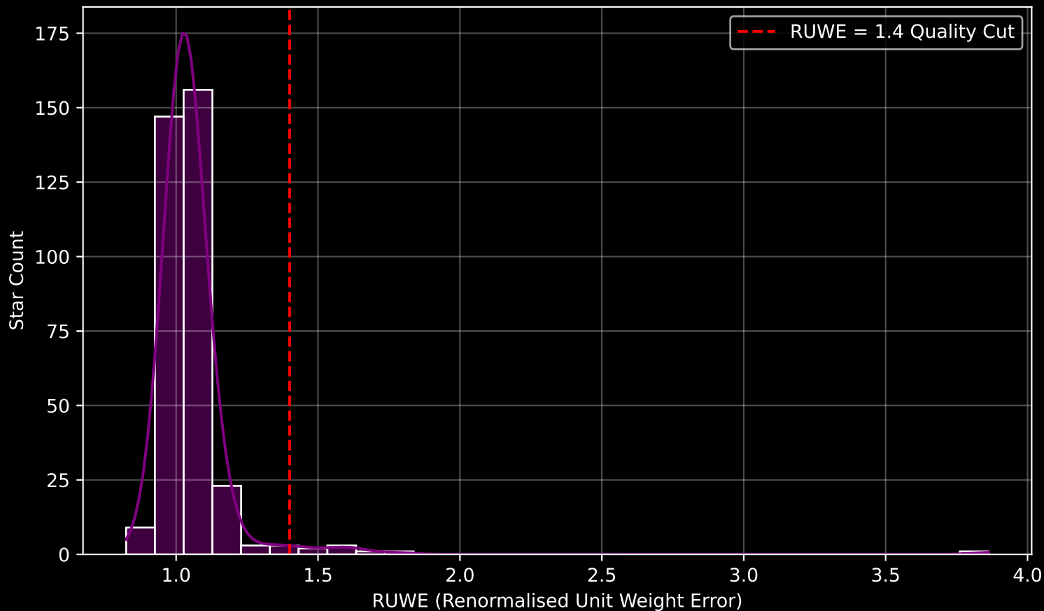
GAPOGEE DR17 Field [140+06] RUWE Distribution (n= 349)
