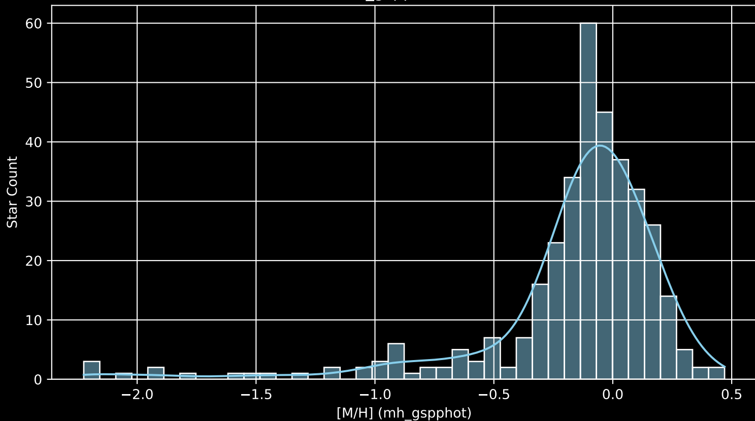
APOGEE DR17 Field: [140+06 [M/H] (mh_gspphot) (n= 349)
