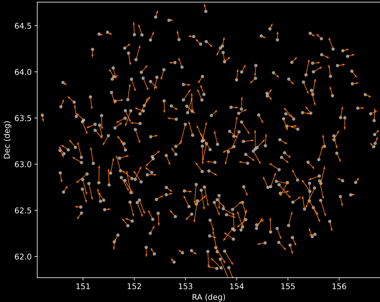
APOGEE DR17 Cluster 2 Proper Motion Vectors (n=275)
